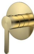
BW0904E Single lever concealed shower mixer Material: 304 Stainless Steel Panel: 304 Stainless Steel Cartridge: 35mm Function: 1
