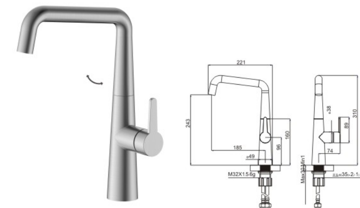
BW7219 Single lever kitchen mixer Material: 304 Stainless Steel Cartridge: 30mm
