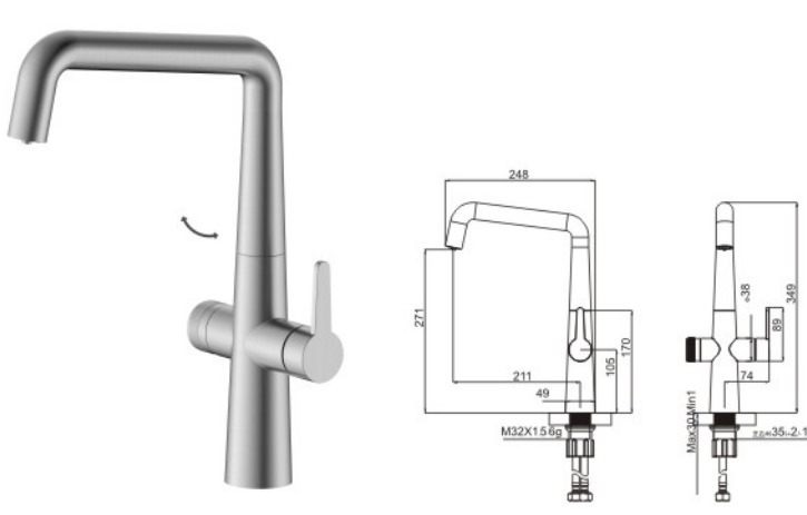
BW7855 Single lever kitchen mixer Material: 304 Stainless Steel Cartridge: 30mm
